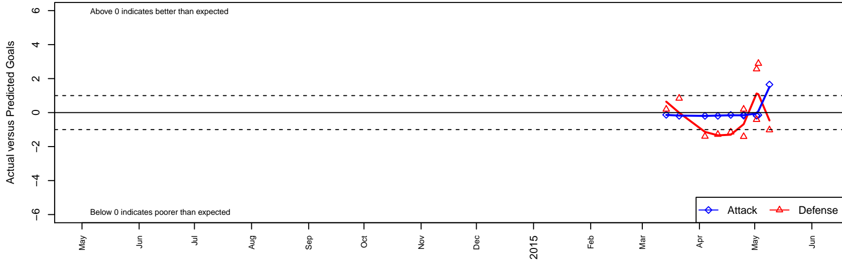
Mountain Home G02 Dots are actual minus expected GF (blue circles) and GA (red triangles). Blue line is smoothed change in attack strength. Red is smoothed change in defense strength.
